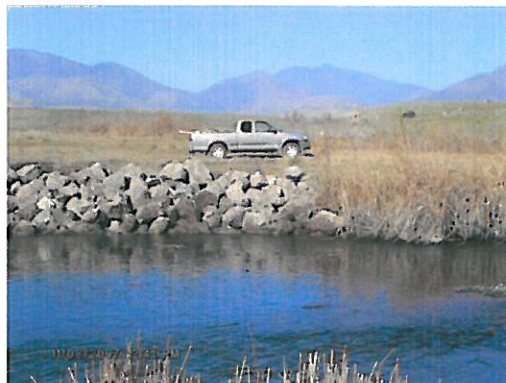
Stream bank armoring upstream from temporary bypass channel inlet (Oct/Nov 2007)
